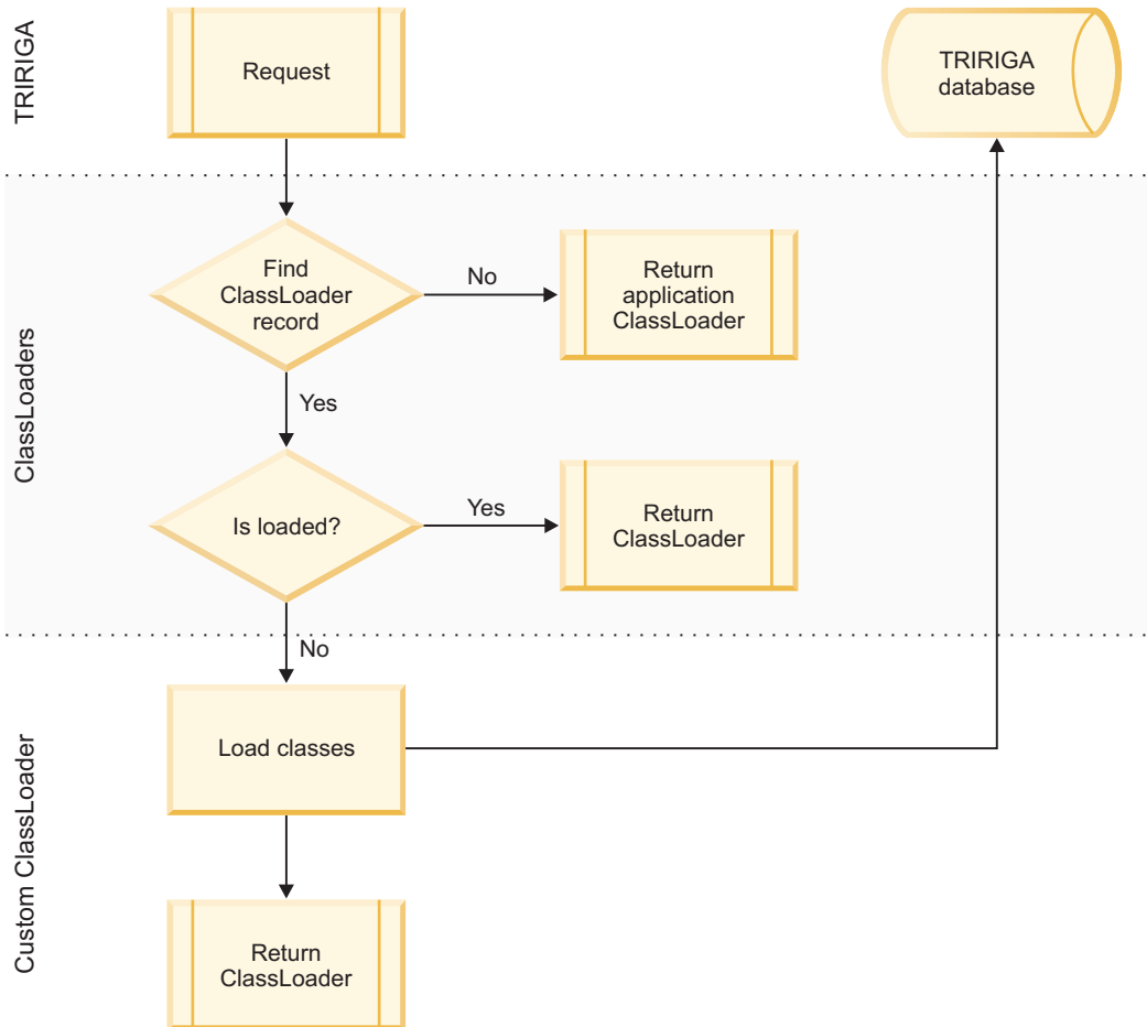
Figure 1. Custom ClassLoader
